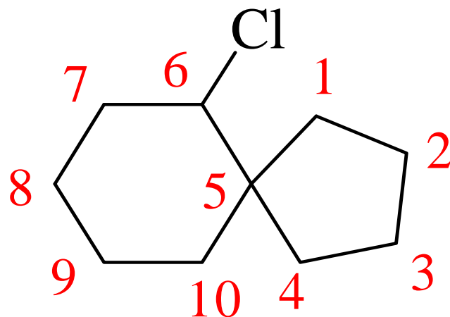
6-氯螺[4.5]癸烷 6-Chlorospiro[4.5]decane
